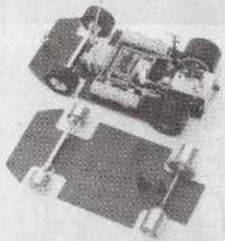
WORKRITE's new deluxe electric racer complete with Marker chassis and Futaba radio.
